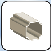
F1515-4 1 1/2" x 1 1/2" FLUTED (0.070" Wall) Corner R.O.125"
