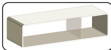
F2080-1 2" x 8" RIBBED RAIL AVAILABLE AS HOLLOW RAIL(NO RIB) (0.090" WALL) CORNER R.O.188"
