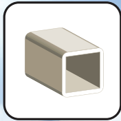
F1515-1 1 1/2" x 1 1/2" PICKET 3/2" or 3/8" (0.120" Wall) Corner R.O.125"
