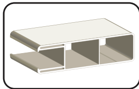
F1555-4 1 1/2" x 5 1/2" POCKET RAIL (0.080" Wall) CORNER R.O.188"
